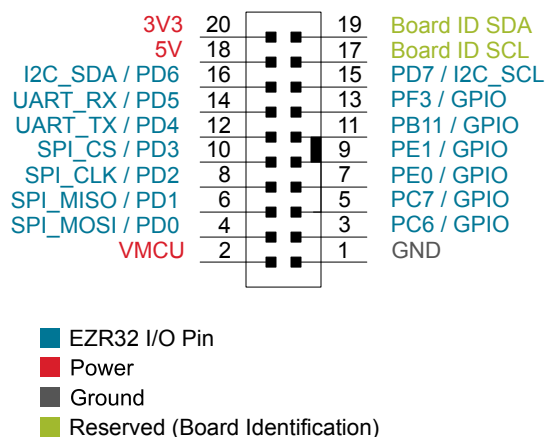
Figure 4.3. Expansion Header
